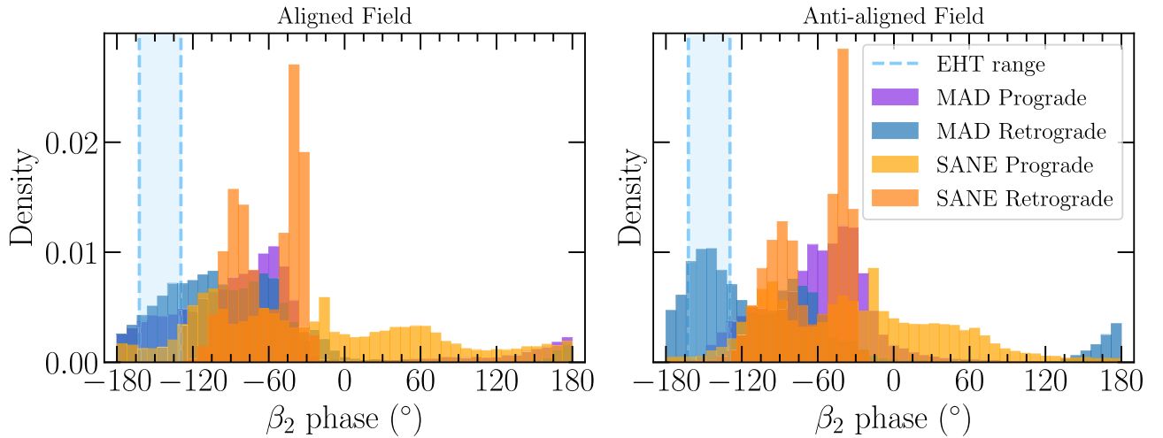
Figure 26. Distribution of \beta_2 phase for an aligned (left panel) and anti-aligned (right panel) magnetic field representing values taken from all images in the EHT M87* library blurred with a 20 \mu\text{as} beam. Allowed inferred ranges of EHT image reconstructions are limited by the dashed lines.
